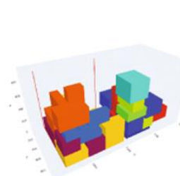
(l) 3dBPP_11: M = 800 ; \eta = 2 and \{0: \text{red}, 7: \text{yellow}\} weight more than twice of the rest; \{7: \text{yellow}, 9: \text{red}\} incompatible; \{(0: \text{red}, 3: \text{teal}), (0: \text{red}, 8: \text{orange})\} together; (\bar{L}, \bar{W}) = (750, 750) .
