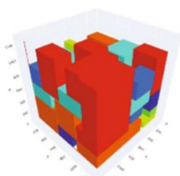
(b) 3dBPP_1: 51 items without restrictions and \sum_{i \in I} \mu_i = 1776 .
