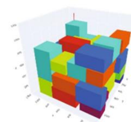
(e) 3dBPP_4: inst. 3dBPP_3 with \eta = 2 . \{0: \text{red}, 1: \text{blue}, 9: \text{red}\} weight more than twice of \{3: \text{teal}, \dots, 8: \text{orange}\} .
