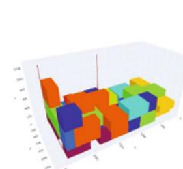
(i) 3dBPP_8: inst. 3dBPP_7 with \{(4: \text{teal}, 8: \text{orange}), (0: \text{red}, 3: \text{teal}), (0: \text{red}, 8: \text{orange})\} together.
